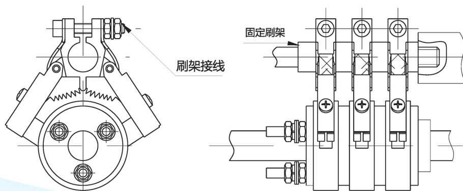
Installation Schematic Diagram
